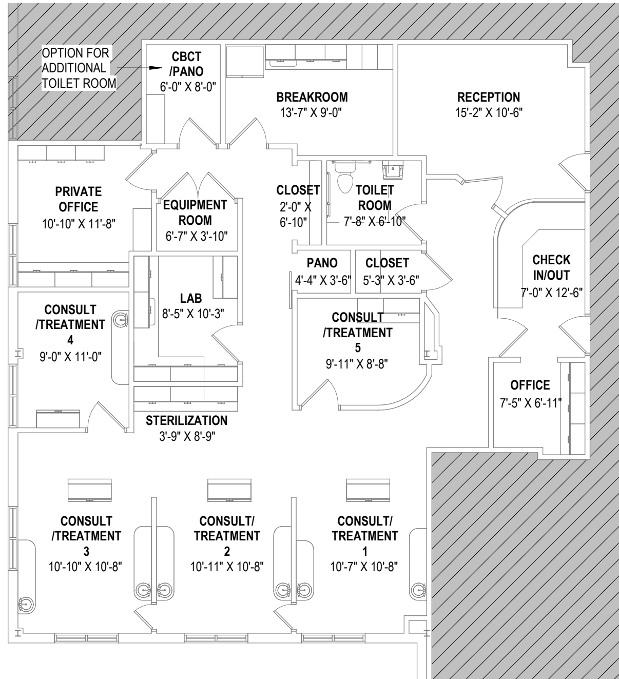
① SUITE F 1/8" = 1'-0"
